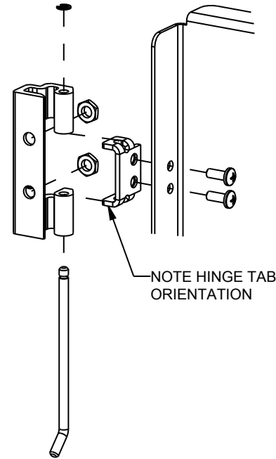
EXPLODED HINGE DETAIL
