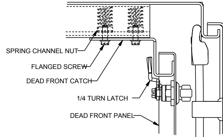
INTERIOR RIGHT SIDE SECTION VIEW
