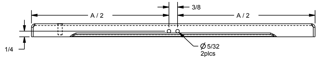
ENCLOSURE DOOR DRILL DETAIL
