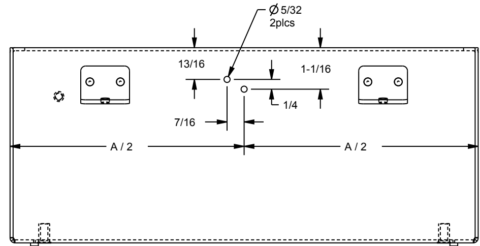
ENCLOSURE BODY DRILL DETAIL
